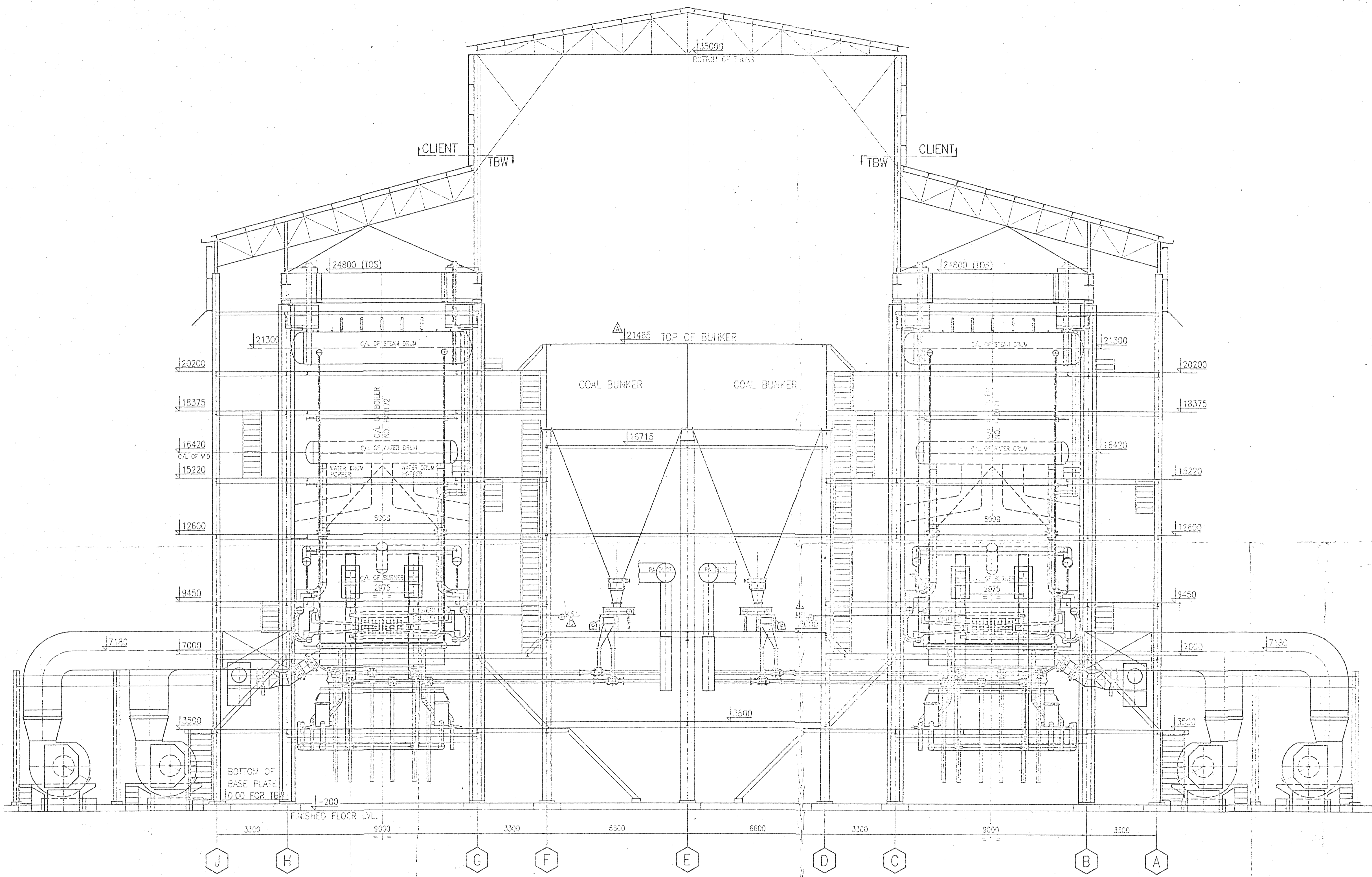
VIEW FROM BOILER FRONT SHOWING BOILER AREA ONLY
